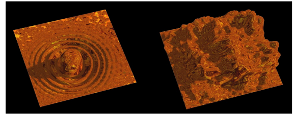
Figure 5: Snapshots of displacement field on top of a plate just after a strike (left) and during fully developed nonlinear state (right), with the presence of large and small wavelengths.
