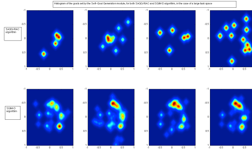
Figure 6: Histograms of the goals set by the Goal Self-Generation Module when the task space is large. The different figures correspond to the results for different runs of the experiment with SAGG-RIAC algorithm (1st row) and SGIM-D algorithm (2nd row). Both rows figures have been zoomed and centred on the reachable space
