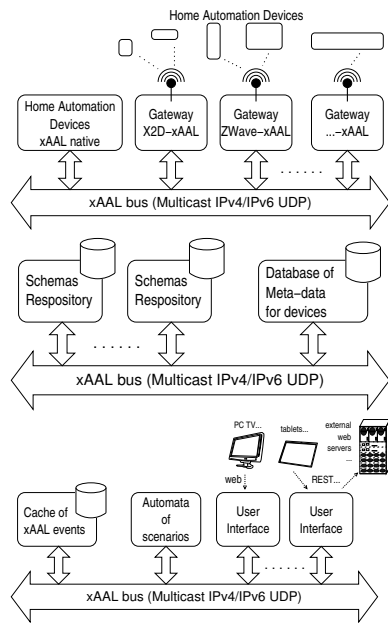
Fig. 3: Functional Architecture of xAAL.
