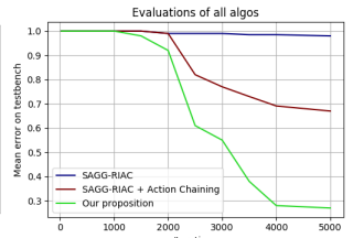
Fig. 5: Learning a hierarchical task: placing objects on the spots, i.e. controlling the observable v
