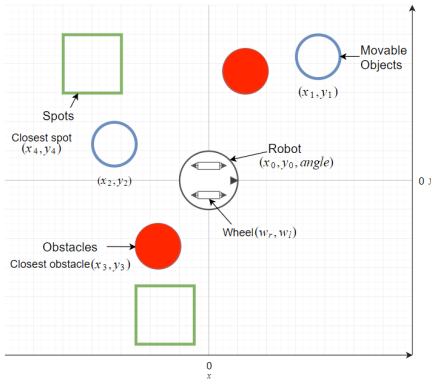
Fig. 3: CHIME experimental setup, (w_r, w_l) are the primitive policy spaces, the outcome spaces are indicated inside parenthesis and a reward outcome value v , depending on whether an object is on a spot or not, is also present.
