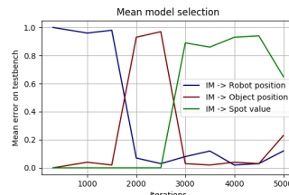
Fig. 4: Mean model selection during learning, based on interest
