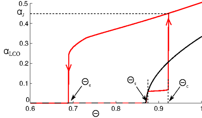
Figure 6: Bifurcation diagram of the 2 dof aeroelastic system with cubic stiffness ( \xi_y = \xi_\alpha = 1 ). Black : without SMA spring. Red : with SMA spring (selected values : h_l = 0.05 , K_1 = 10 K_2 and A_{SMA} = 2.35 \times 10^{-3} )
