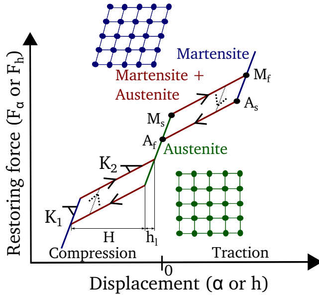
Figure 3: Pseudo-elastic behaviour of SMA and its microstructure for each phase.
