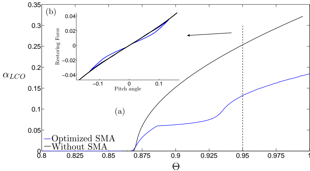
Figure 8: (a) Bifurcation diagram with h_l = 0.05 , K_1/K_2 = 1.5 and \xi_\alpha = 3.4 . (b) Restoring force at \Theta = 0.95 .
