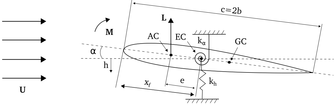
Figure 1: Sketch of the airfoil model as a rigid body in uniform flow U with two dof : pitch ( \alpha ) and heave ( h ).
