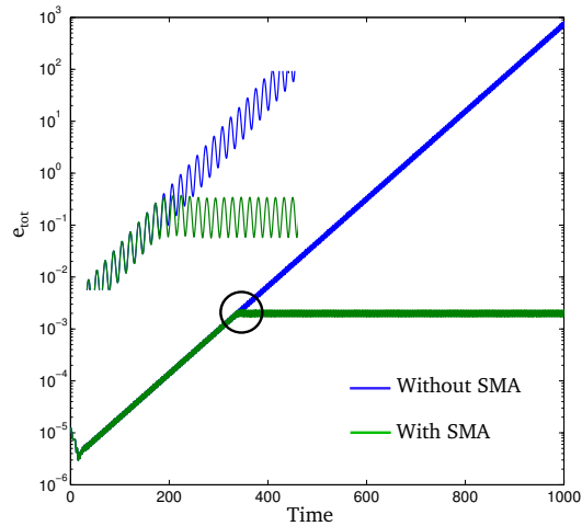
Figure 5: Total energy e_{tot} versus time for the aeroelastic system (parameters of Table 1), with and without SMA, and for \Theta = 0.9 .
