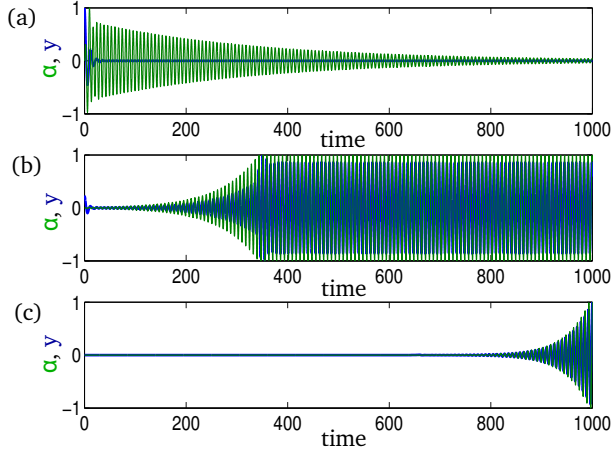
Figure 4: Effect of the SMA on the linear flutter instability ( \xi_y = \xi_\alpha = 0 ) for three different reduced velocities: (a) Linear stability case, \Theta = 0.86 (b) Instability case, with LCO due to SMA dissipation, \Theta = 0.91 (c) Instability case where SMA cannot dissipate enough energy, and an exponential growth is observed, \Theta = 0.93 ( \Theta_f = 0.87 and \Theta_c = 0.926 ). Blue : heave motion y , green : pitch \alpha . The curves are normalized to their maximal value.
