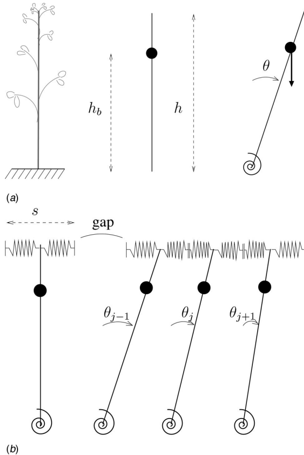
Fig. 1 (a) Schematic view of the stem model, a straight rod of height h , with a point mass at the height h_b , subjected to gravity and a restoring moment from a torsional spring at the basis of the rod. (b) Schematic view of the stem interaction model. A spring is added on the rod, to simulate the foliage. Depending on the angles of two adjacent stems, they can be in contact or there can be a gap.
