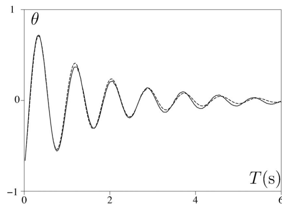
Fig. 3 Stem angular position as a function of time, experiment (solid line) and theory (dashed line)
