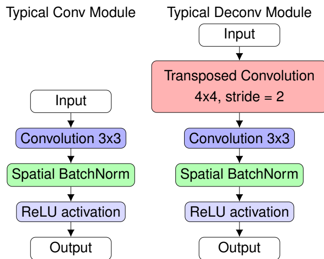
Figure 3.9: General Structure of convolution and deconvolution blocks of DepthNet.
